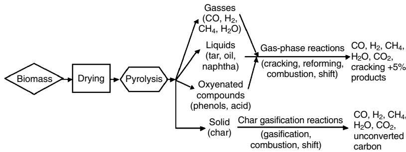
FIGURE 5.2 Potential paths for gasification.
