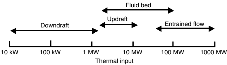
FIGURE 6.2 Range of applicability for biomass gasifier types.
