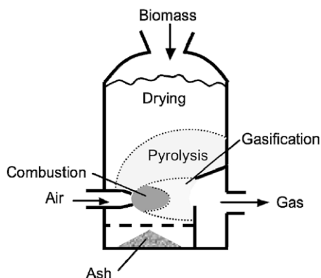
FIGURE 6.7 Schematic of a crossdraft gasifier.
