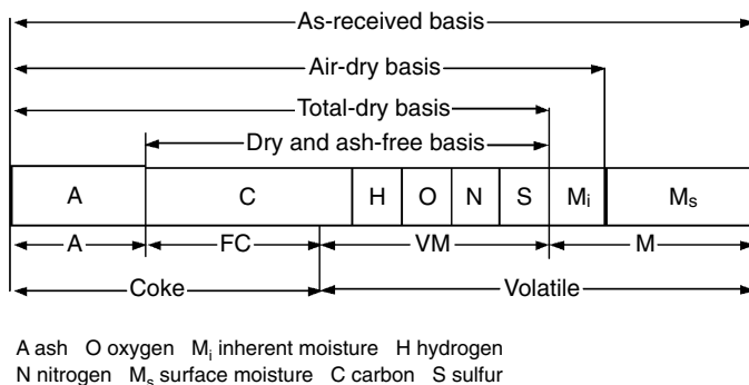
FIGURE 2.14 Bases for expressing fuel composition.
