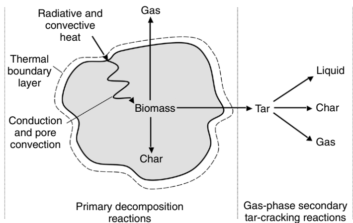
FIGURE 3.4 Pyrolysis in a biomass particle.
