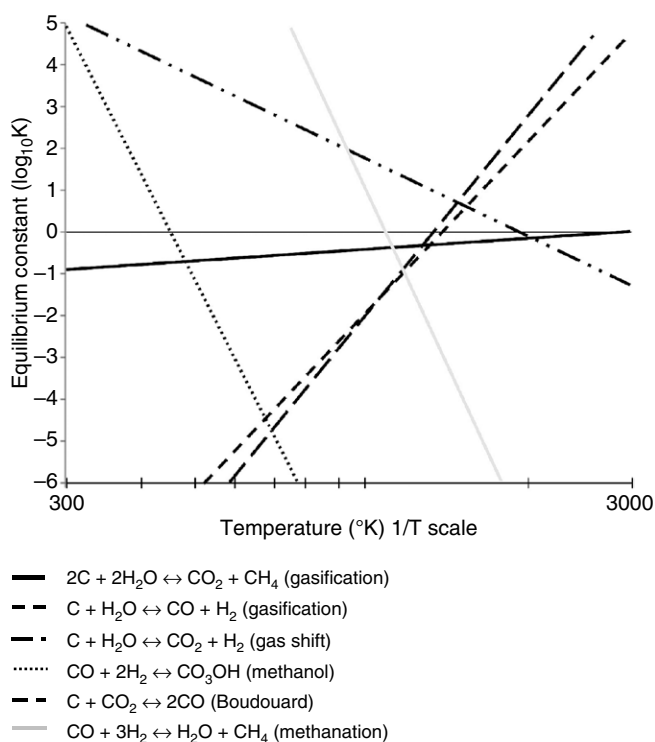
FIGURE 5.4 Equilibrium constants for selected gasification reactions. (Source: Adapted from Probstein and Hicks, 2006, p. 63.)
