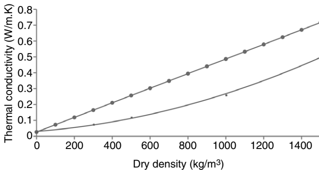
FIGURE 2.13 Thermal conductivity of biomass along the grain and across the grain increases with dry density. The plot is for dry wood. (Source: Adapted from Thunman and Leckner, 2002.)
