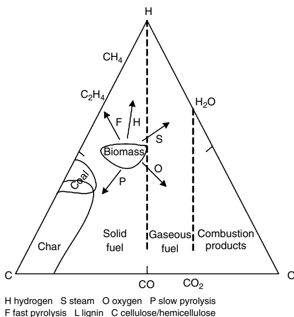
FIGURE 2.12 C-H-O ternary diagram of biomass showing the gasification process.
