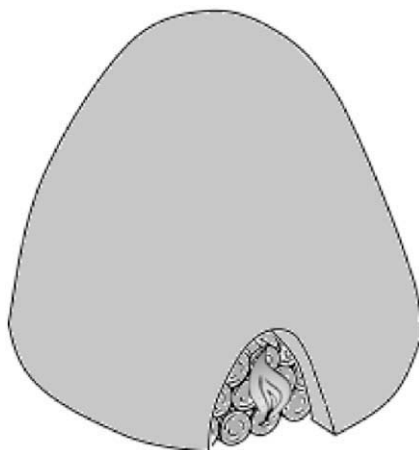
FIGURE 3.2 Beehive oven for charcoal production through slow pyrolysis of wood.
