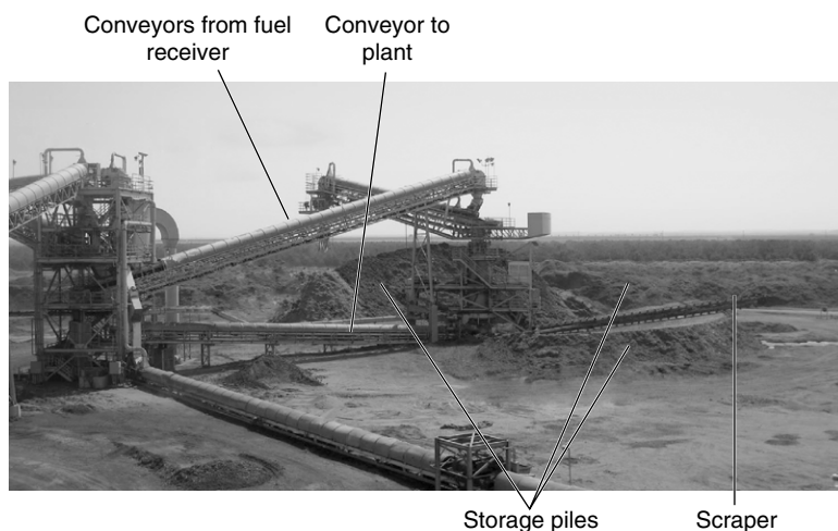
FIGURE 8.4 Biomass is conveyed to the storage pile; the scraper collects it when needed and transfers it to conveyors that take it to the fuel preparation plant. (Source: Photograph by the author.)
