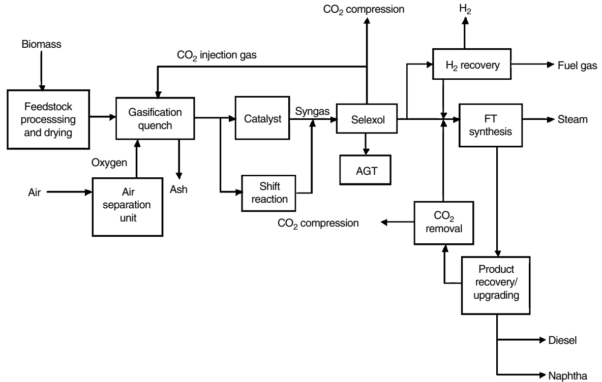
FIGURE 9.6 Transport fuel production from coal and biomass using Fisher-Tropsch synthesis. (Source: Adapted from White et al. , 2007.)
